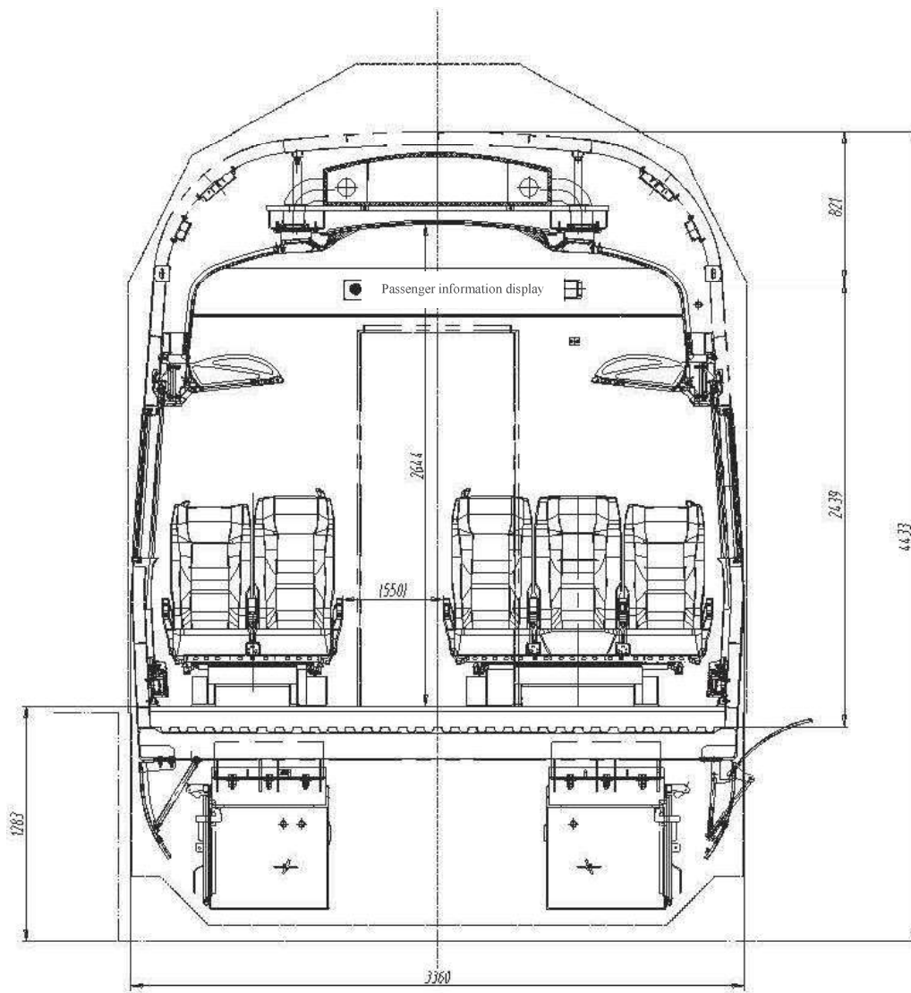
Figure II Section Layout of Control Car (Economy-class Seat)
