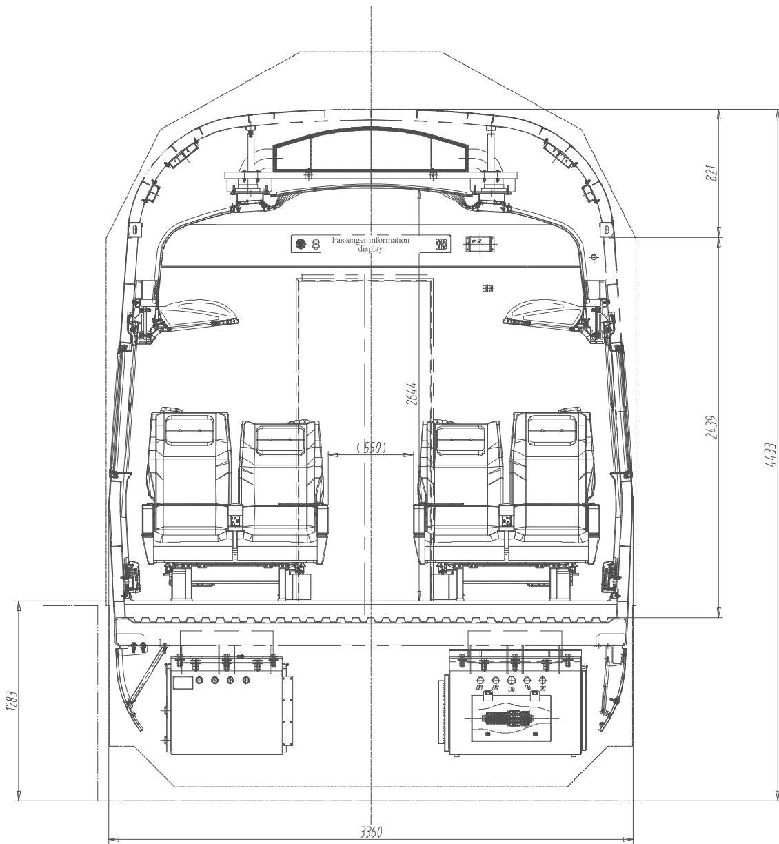
Figure IV Section Layout of Control Car (business-class Seat)
